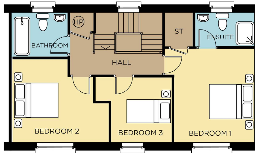
TYPE B - FIRST FLOOR
